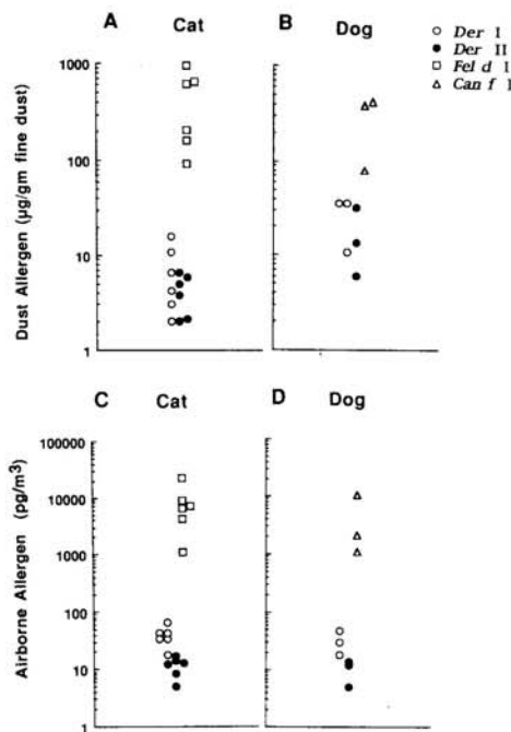
FIG. 1. Floor dust and airborne allergens in living rooms during routine activities. A, Floor dust allergens in houses with cats; B, floor dust allergens in houses with dogs; C, airborne allergens in houses with cats; D, airborne allergens in houses with dogs.
