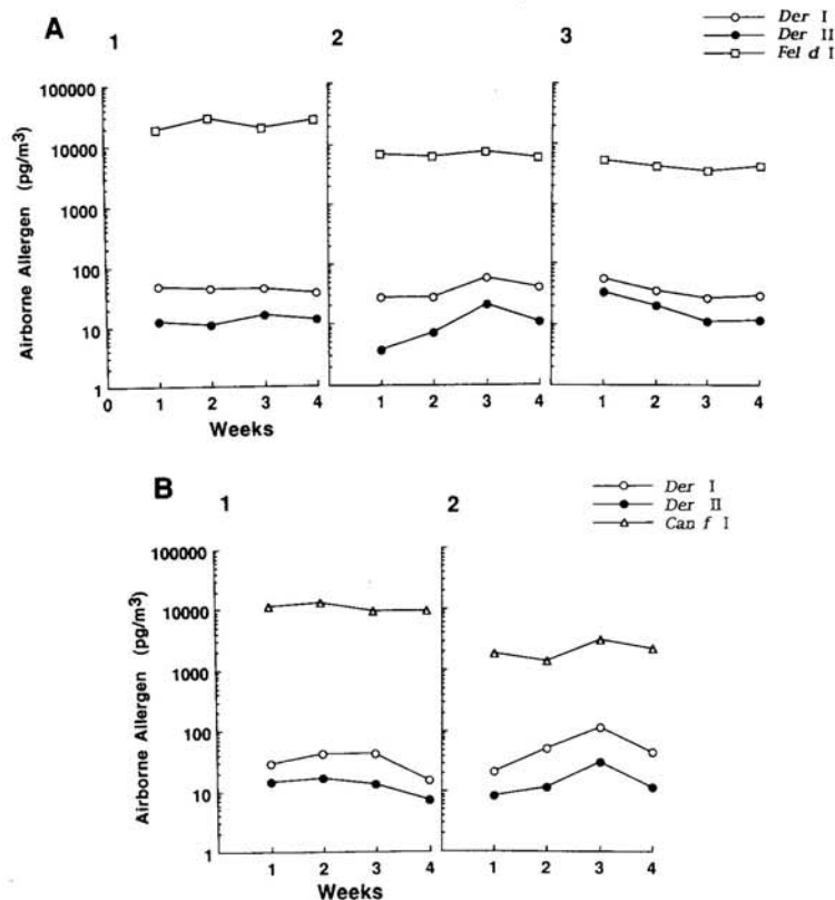
FIG. 2. Weekly measurements of airborne allergen levels in living rooms during routine activities. A , Houses with cats: 1, house F in Table I; 2, house G; 3, house H. B , Houses with dogs: 1, house L in Table I; 2, house M.
